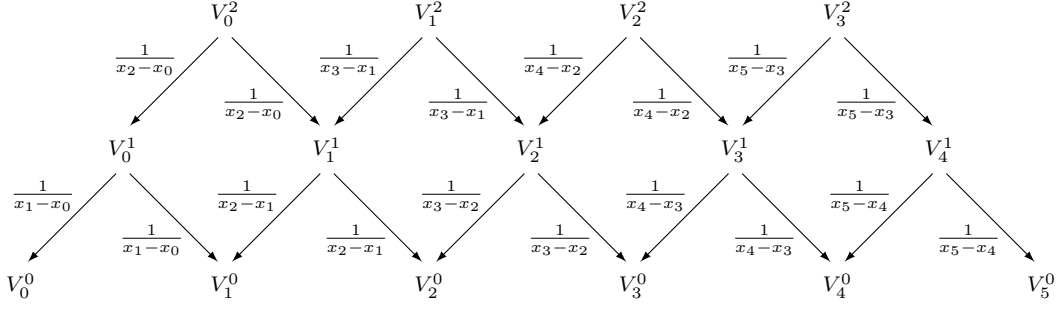
Figure 5: Example of the pyramid algorithm for computing the Floater–Hormann weights w_i in (3) with n = 5 and d = 2 .
