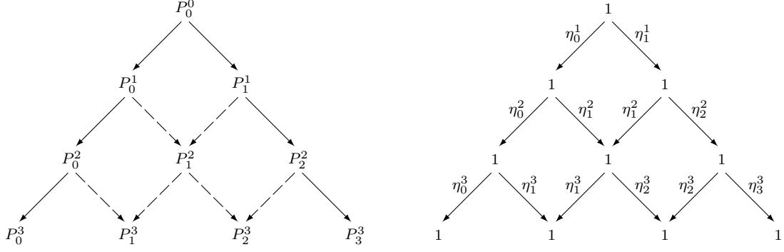
Figure 3: Recurrence of the values P_i^\ell (left), which are all equal to 1 (right).
