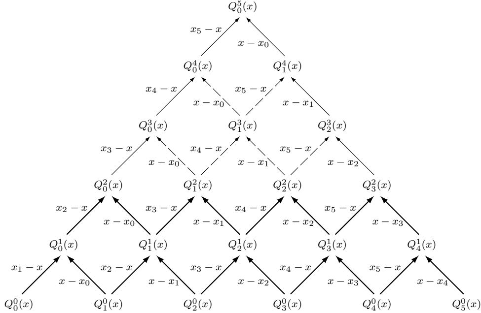
Figure 2: Example of the pyramid algorithm for Floater–Hormann interpolation with n = 5 and d = 2 .
