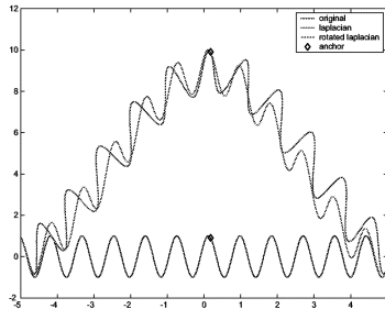
Fig. 2. The differential coordinates are not rotation-invariant. Therefore, when we edit the mesh (lower curve), the orientation of the details with respect to the low-frequency surface is not preserved. To rectify this, we explicitly rotate the differential coordinates (see the dark curve).
