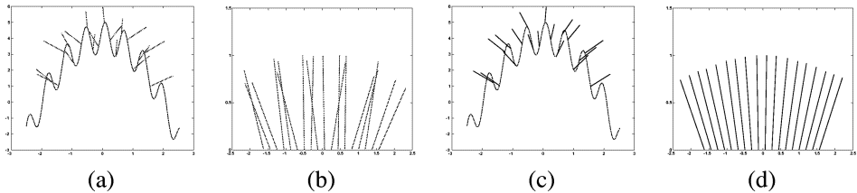
Fig. 5. A 2D example of smooth surface normals estimation. (a) and (c) show the surface with high-frequency detail and the estimated normals of the underlying smooth surface. In (a) a naive averaging of the detailed surface normals was used. (b) shows the same normal vectors as in (a), but the y coordinate of the origin point of each normal is set to zero. This visualizes the problem of the naive estimation - the resulting normals do not vary smoothly. In (c) we show the result of normals estimation using weighted average (with the same support as in (a)–(b)), as explained in Section 7. As demonstrated in (d), such estimation leads to more smoothly-varying normals which are closer to the real smooth surface normals.
