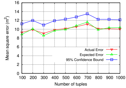
Fig. 5. Prediction Reliability
